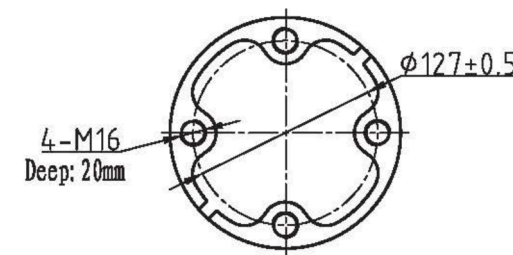
Top & Bottom installation holes
