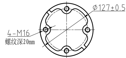
Top & Bottom installation holes
